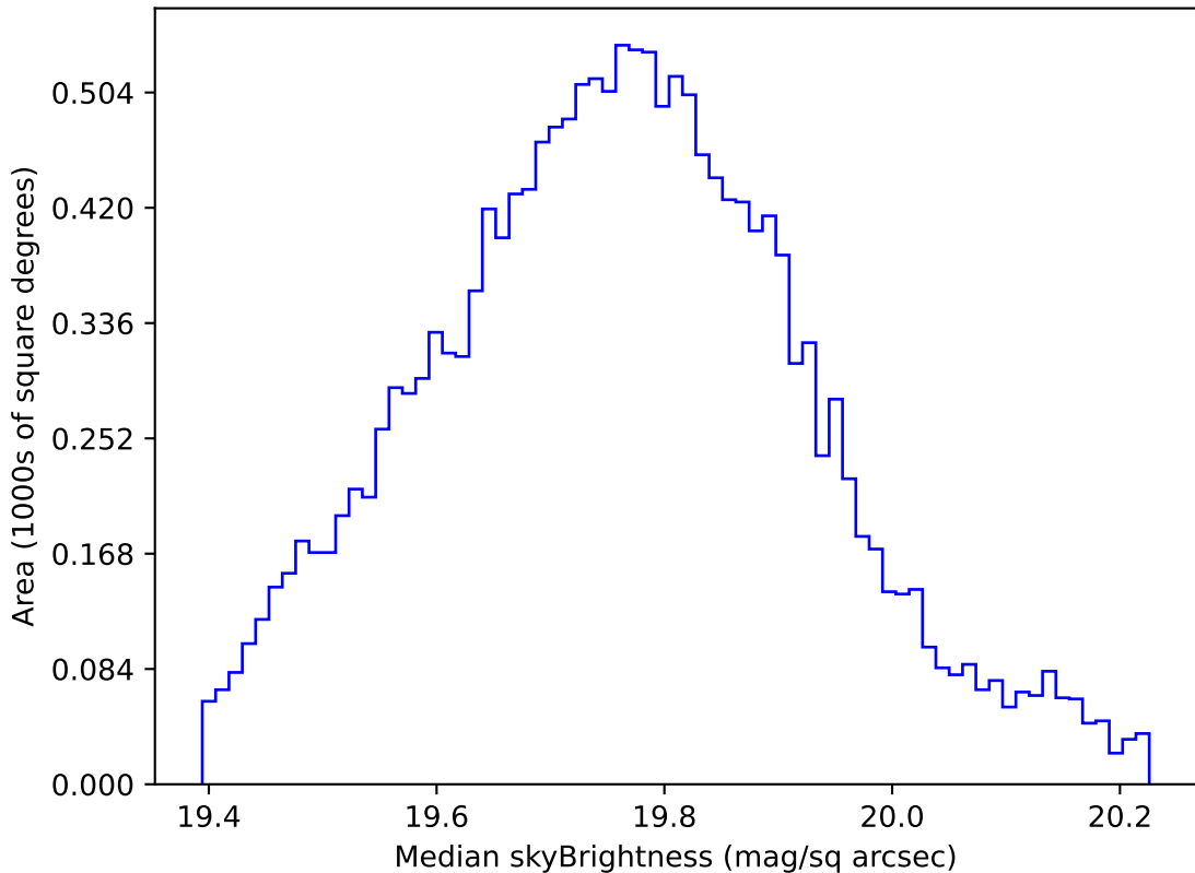
too_elab_r128_d3_gz_v3.4_10yrs WFD all bands: Median skyBrightness
