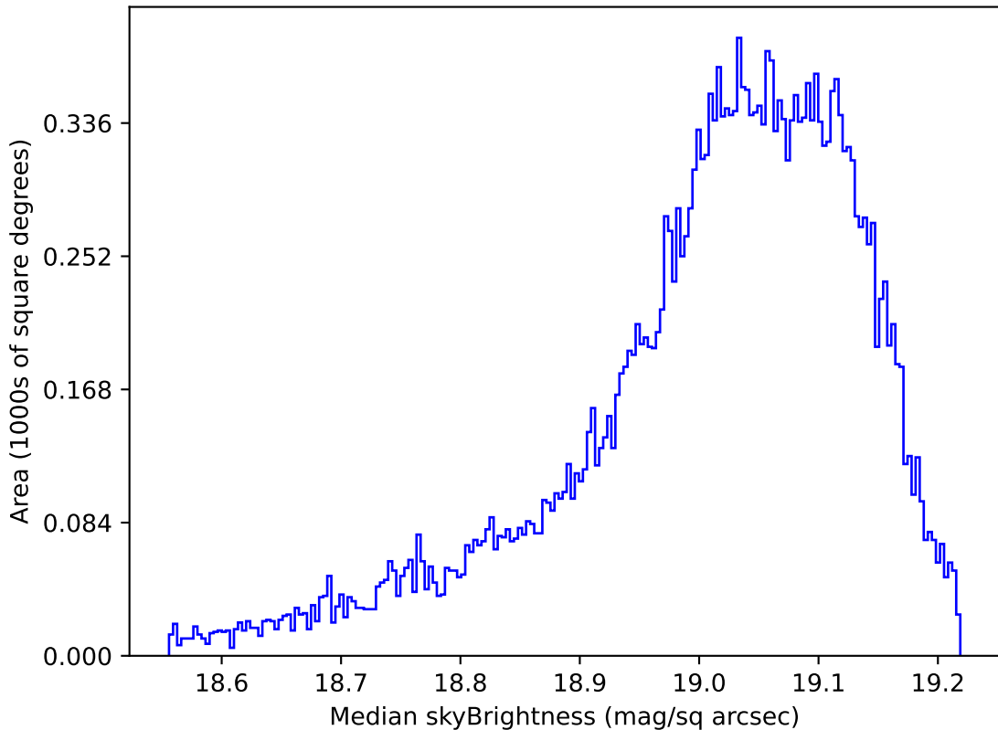
too_elab_r128_d3_gz_v3.4_10yrs All sky z band: Median skyBrightness
