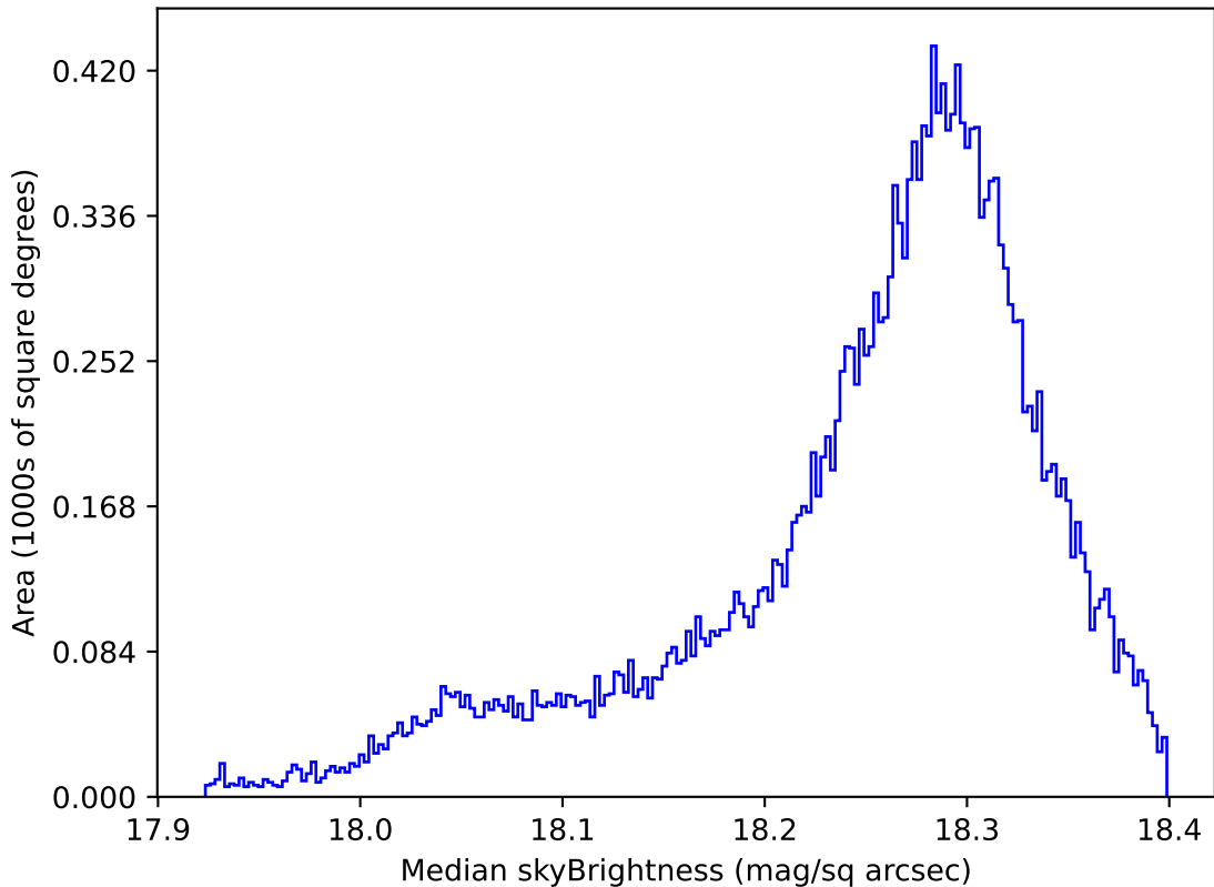
too_elab_r128_d3_gz_v3.4_10yrs All sky y band: Median skyBrightness
