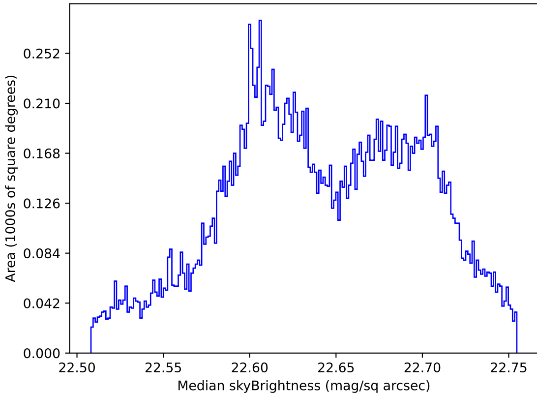
too_elab_r128_d3_gz_v3.4_10yrs All sky u band: Median skyBrightness
