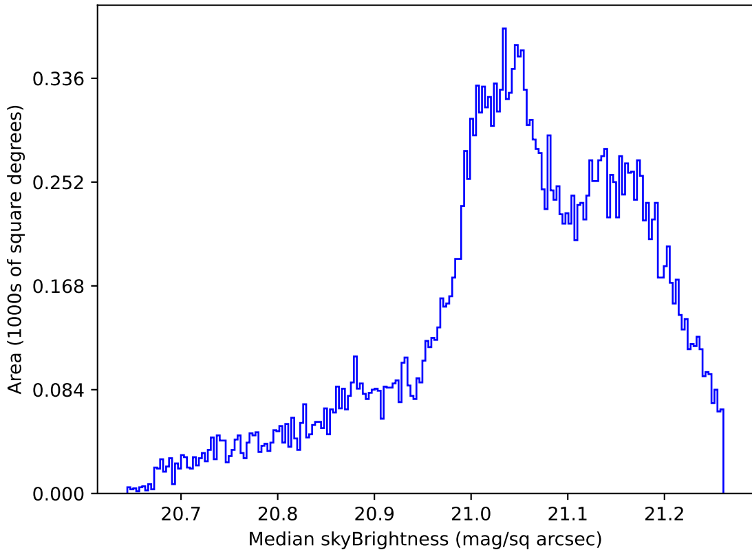
too_elab_r128_d3_gz_v3.4_10yrs All sky r band: Median skyBrightness
