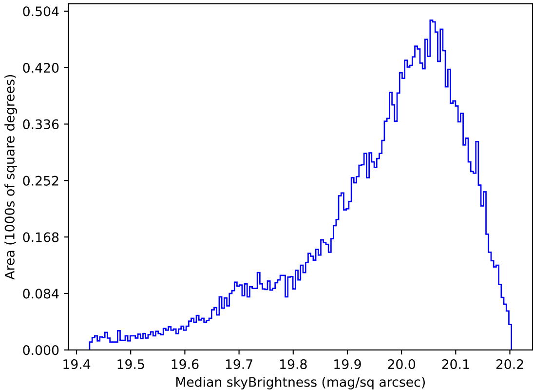
too_elab_r128_d3_gz_v3.4_10yrs All sky i band: Median skyBrightness
