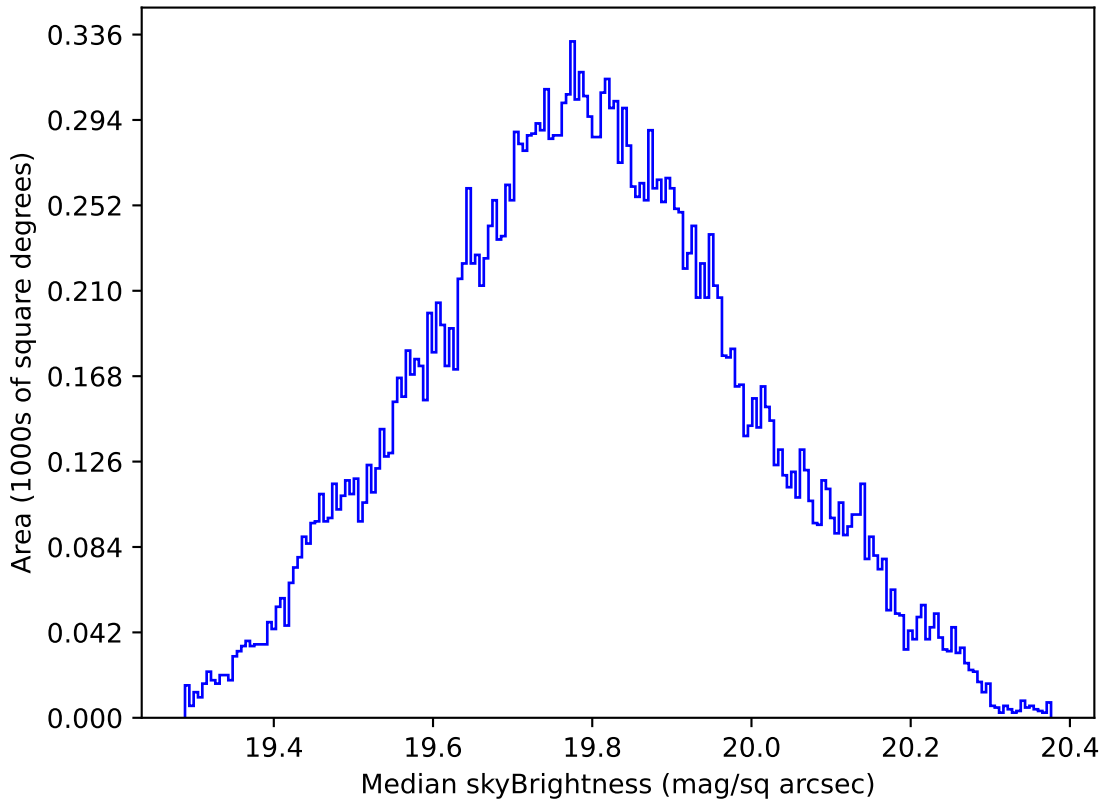
too_elab_r128_d3_gz_v3.4_10yrs All sky all bands: Median skyBrightness
