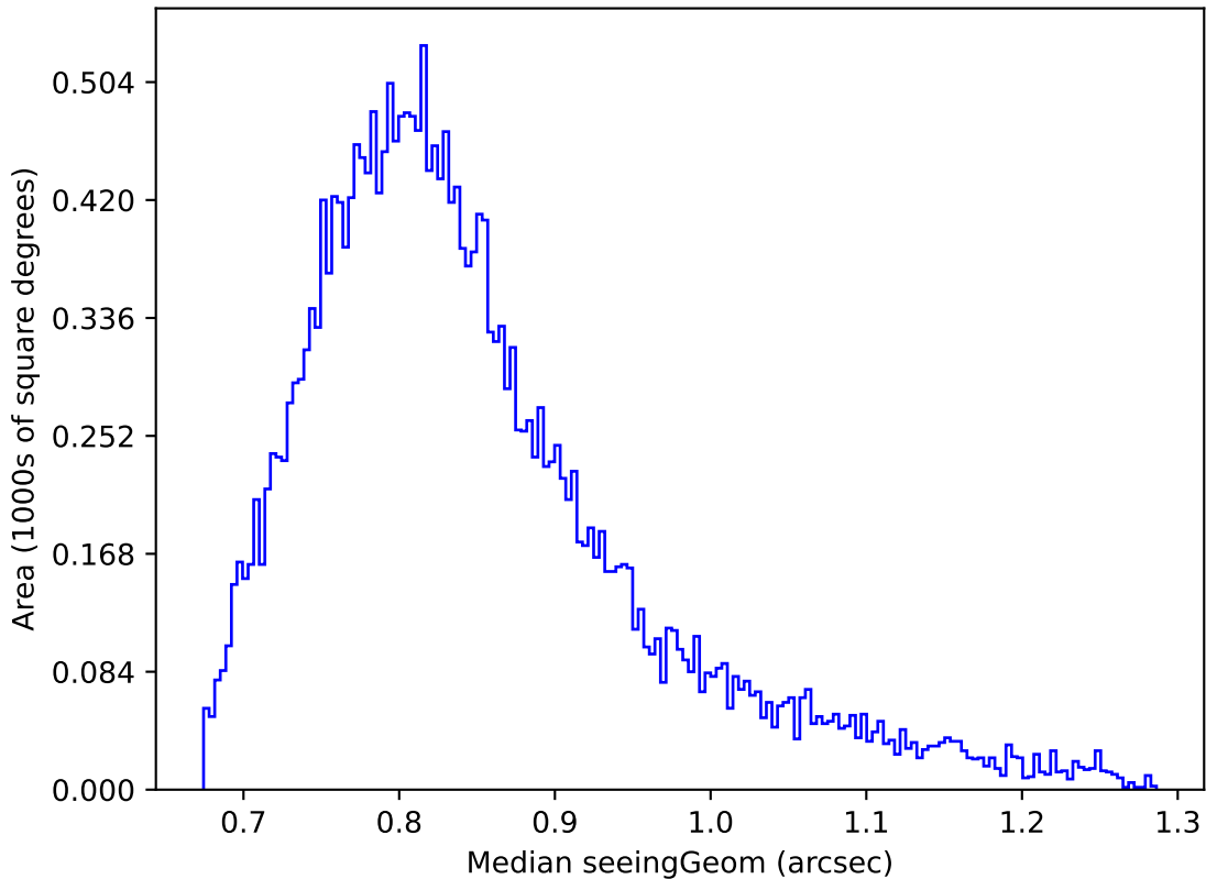
too_elab_r128_d3_gz_v3.4_10yrs Yr 1 z band: Median seeingGeom
