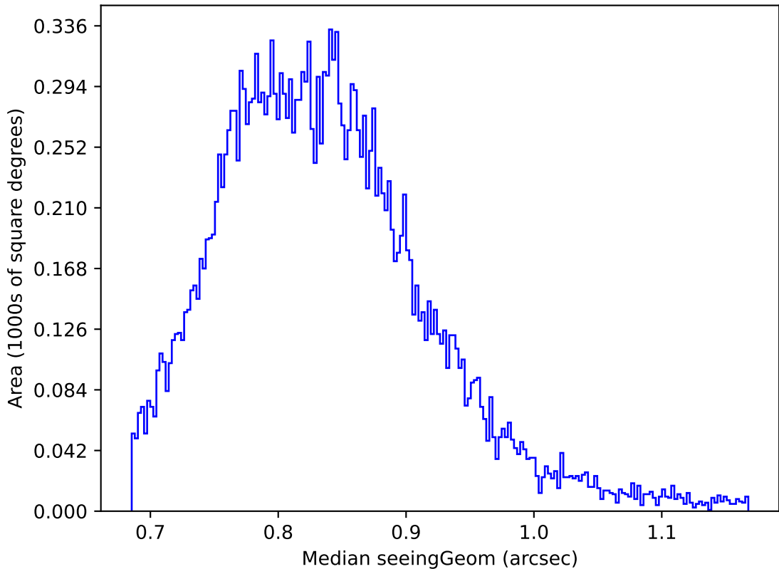
too_elab_r128_d3_gz_v3.4_10yrs Yr 1 y band: Median seeingGeom
