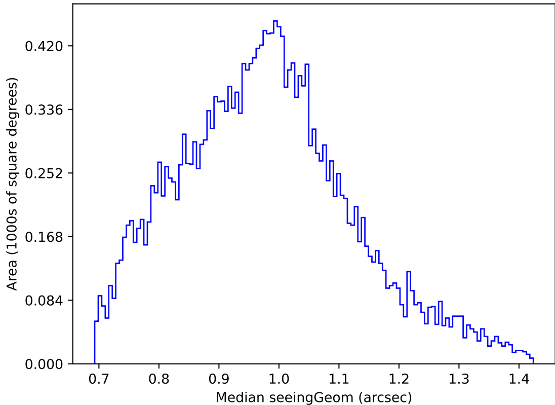
too_elab_r128_d3_gz_v3.4_10yrs Yr 1 u band: Median seeingGeom
