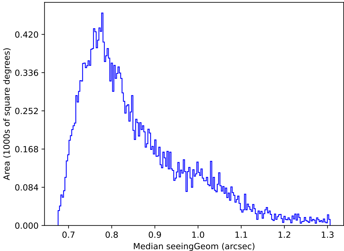
too_elab_r128_d3_gz_v3.4_10yrs Yr 1 r band: Median seeingGeom
