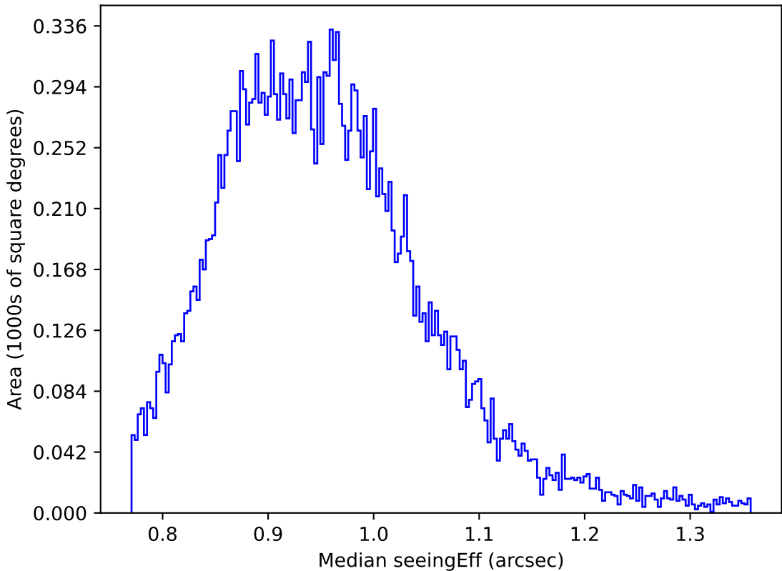
too_elab_r128_d3_gz_v3.4_10yrs Yr 1 y band: Median seeingEff
