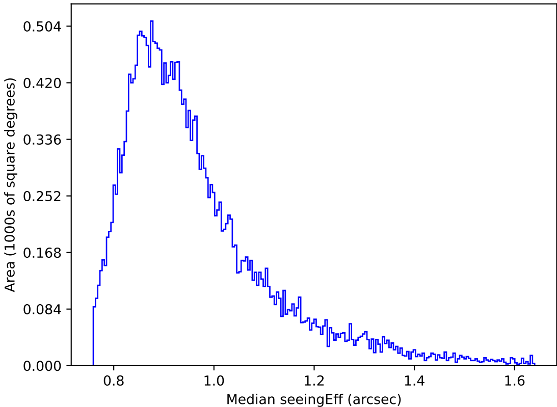
too_elab_r128_d3_gz_v3.4_10yrs Yr 1 i band: Median seeingEff
