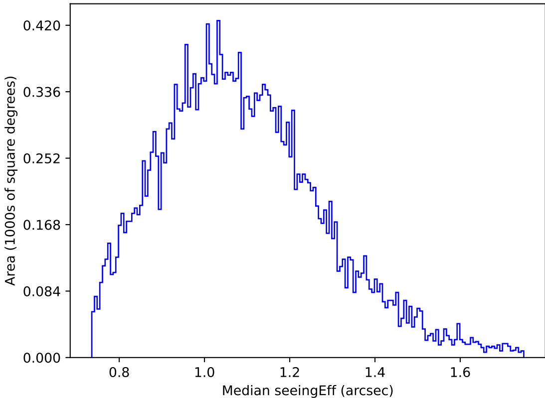
too_elab_r128_d3_gz_v3.4_10yrs Yr 1 g band: Median seeingEff
