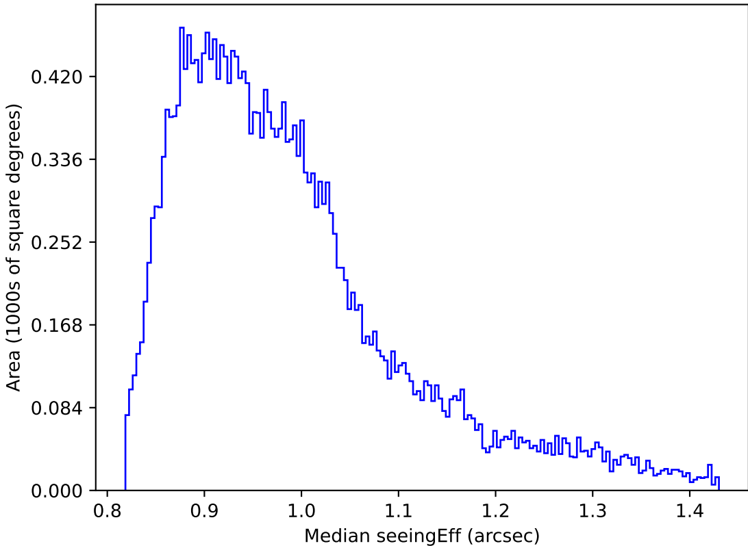
too_elab_r128_d3_gz_v3.4_10yrs Yr 1 all bands: Median seeingEff
