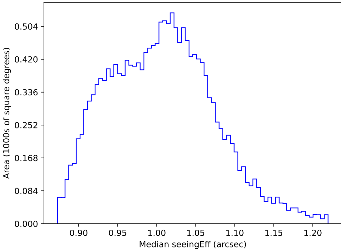
too_elab_r128_d3_gz_v3.4_10yrs WFD z band: Median seeingEff
