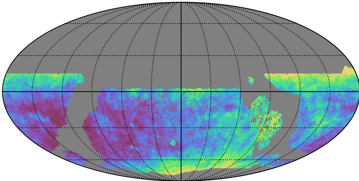
too_elab_r128_d3_gz_v3.4_10yrs WFD y band: Median seeingEff
