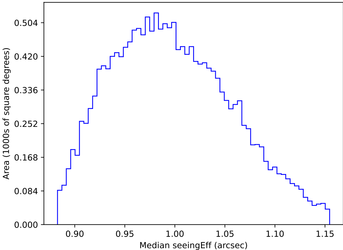
too_elab_r128_d3_gz_v3.4_10yrs WFD y band: Median seeingEff
