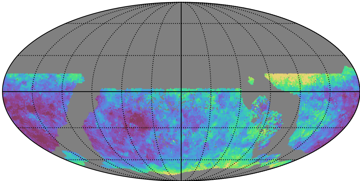
too_elab_r128_d3_gz_v3.4_10yrs WFD u band: Median seeingEff
