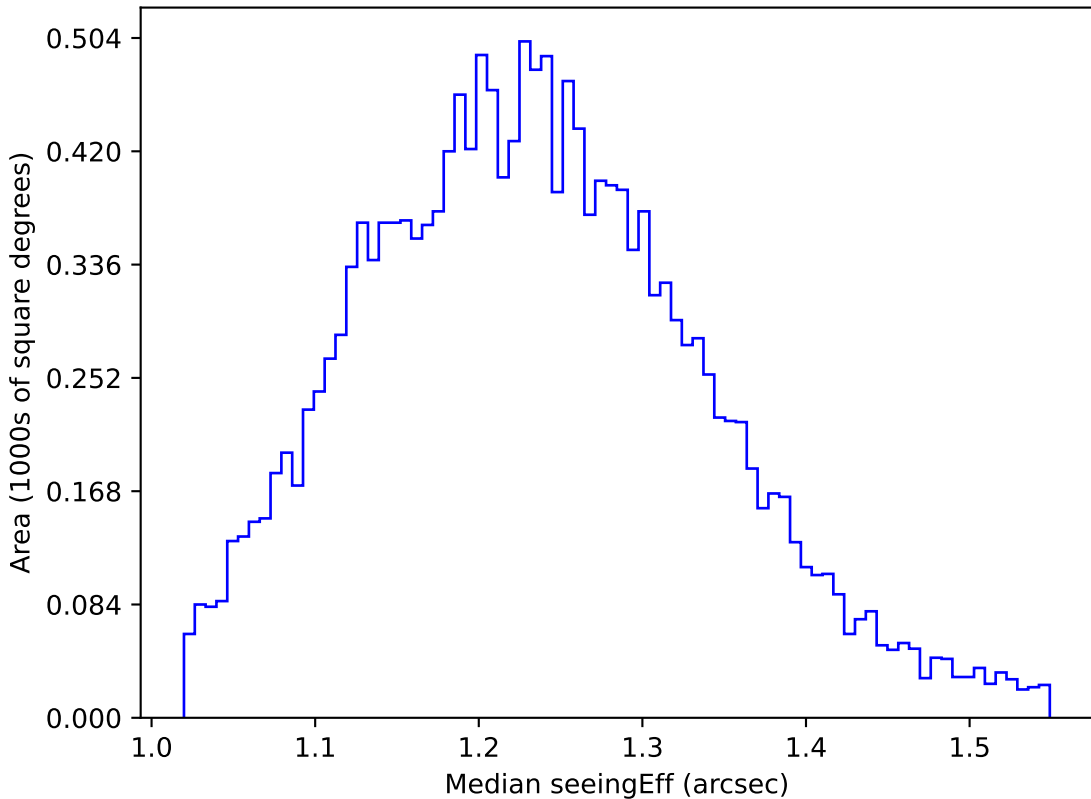
too_elab_r128_d3_gz_v3.4_10yrs WFD u band: Median seeingEff
