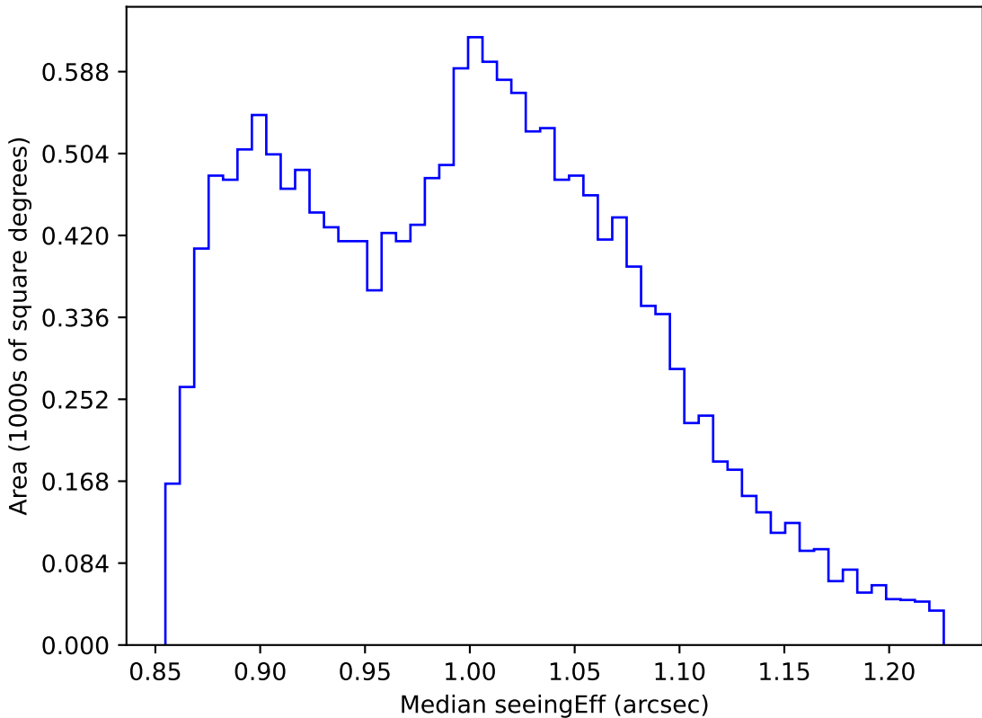
too_elab_r128_d3_gz_v3.4_10yrs WFD i band: Median seeingEff
