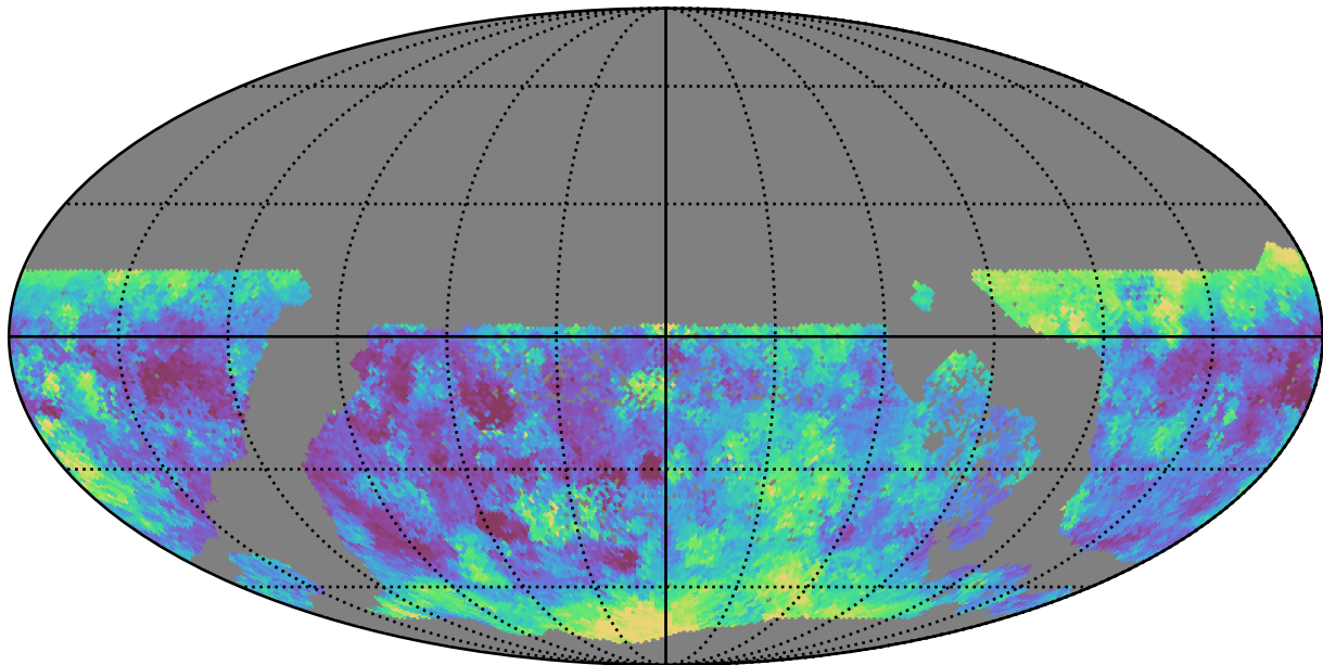
too_elab_r128_d3_gz_v3.4_10yrs WFD g band: Median seeingEff
