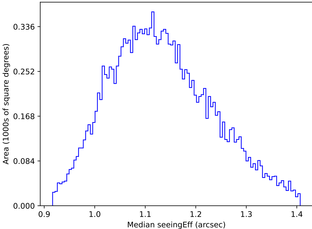
too_elab_r128_d3_gz_v3.4_10yrs WFD g band: Median seeingEff
