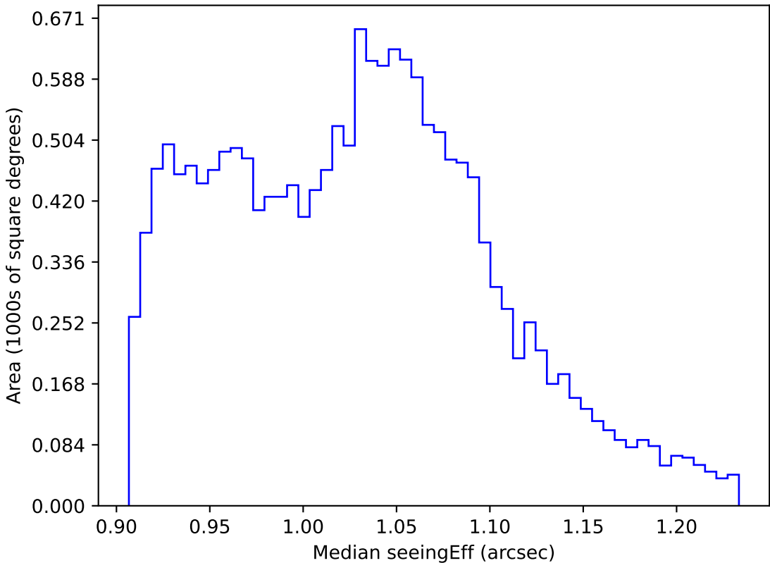
too_elab_r128_d3_gz_v3.4_10yrs WFD all bands: Median seeingEff
