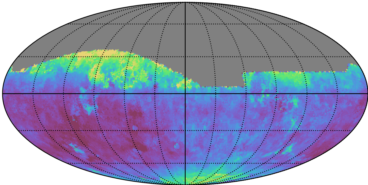
too_elab_r128_d3_gz_v3.4_10yrs All sky z band: Median seeingEff
