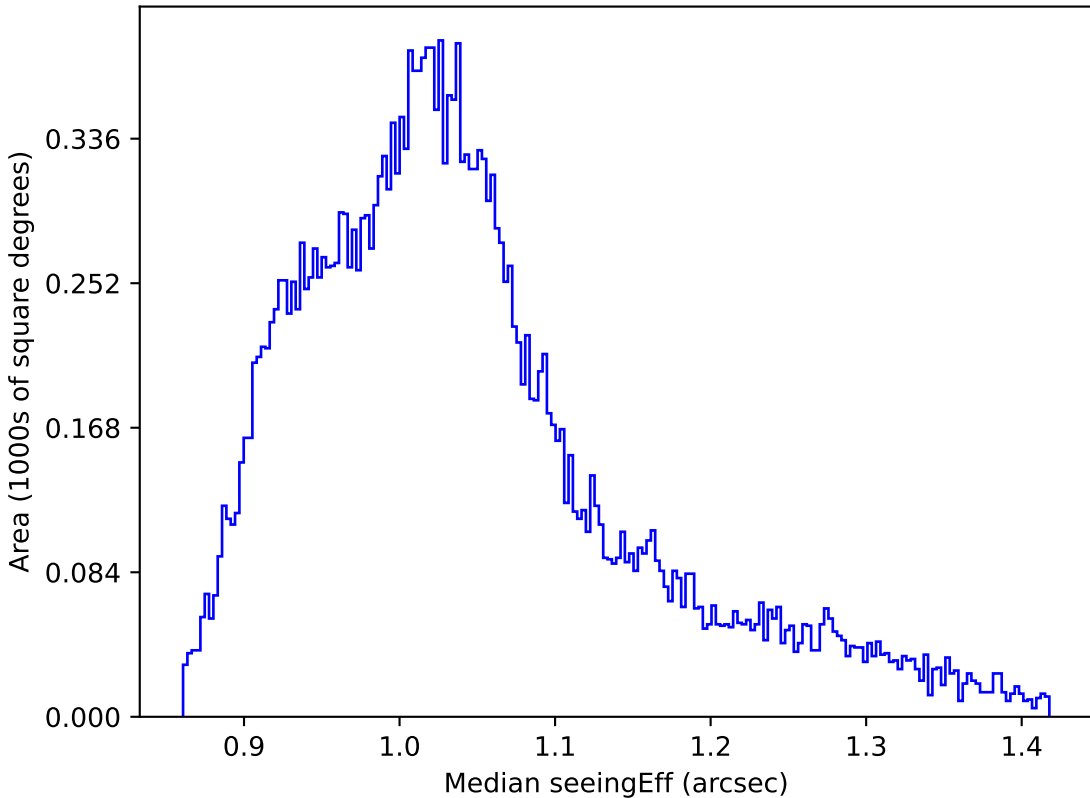
too_elab_r128_d3_gz_v3.4_10yrs All sky z band: Median seeingEff
