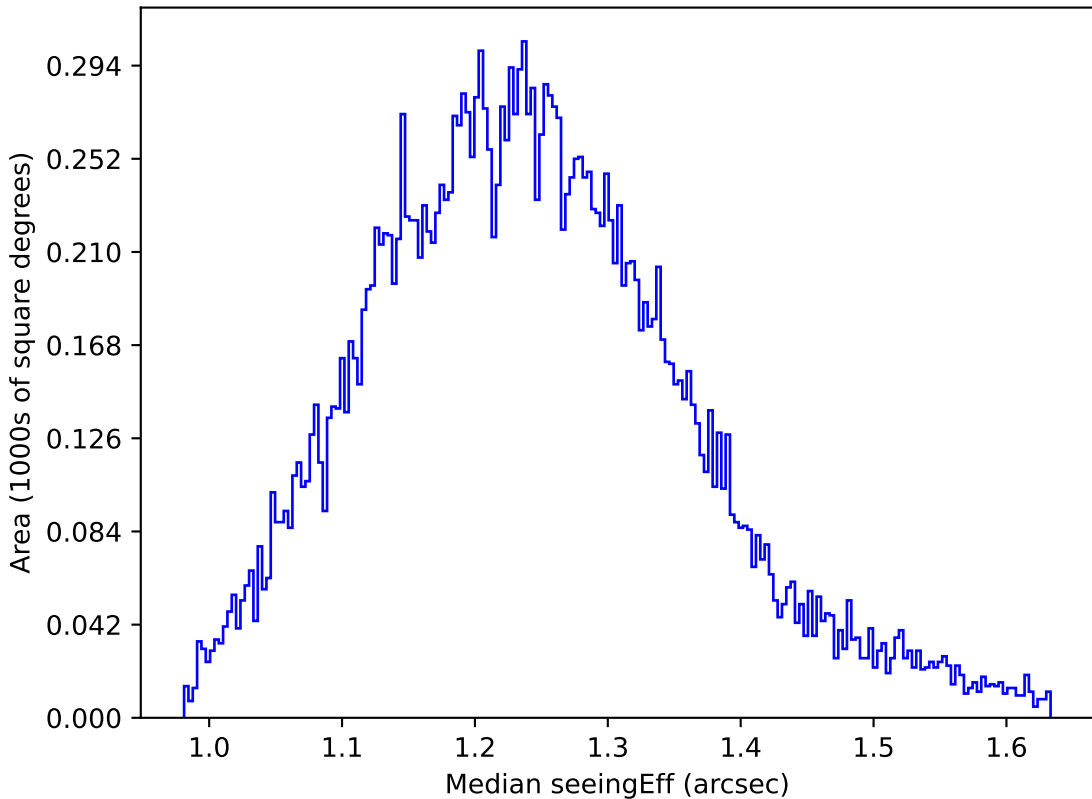
too_elab_r128_d3_gz_v3.4_10yrs All sky u band: Median seeingEff
