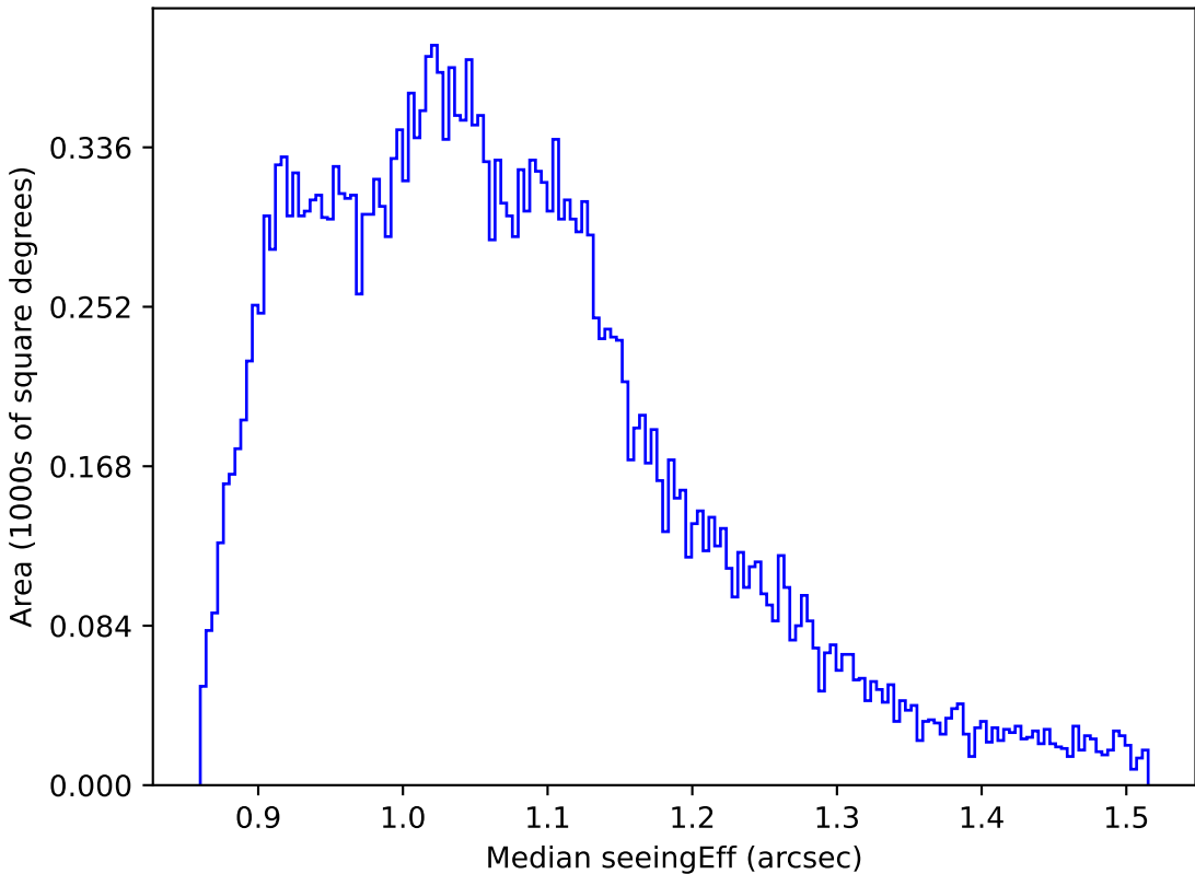
too_elab_r128_d3_gz_v3.4_10yrs All sky r band: Median seeingEff
