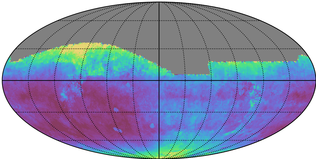
too_elab_r128_d3_gz_v3.4_10yrs All sky i band: Median seeingEff
