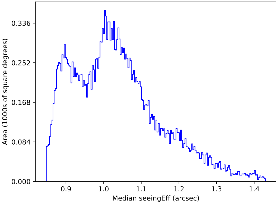
too_elab_r128_d3_gz_v3.4_10yrs All sky i band: Median seeingEff
