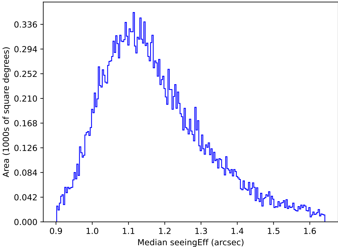
too_elab_r128_d3_gz_v3.4_10yrs All sky g band: Median seeingEff
