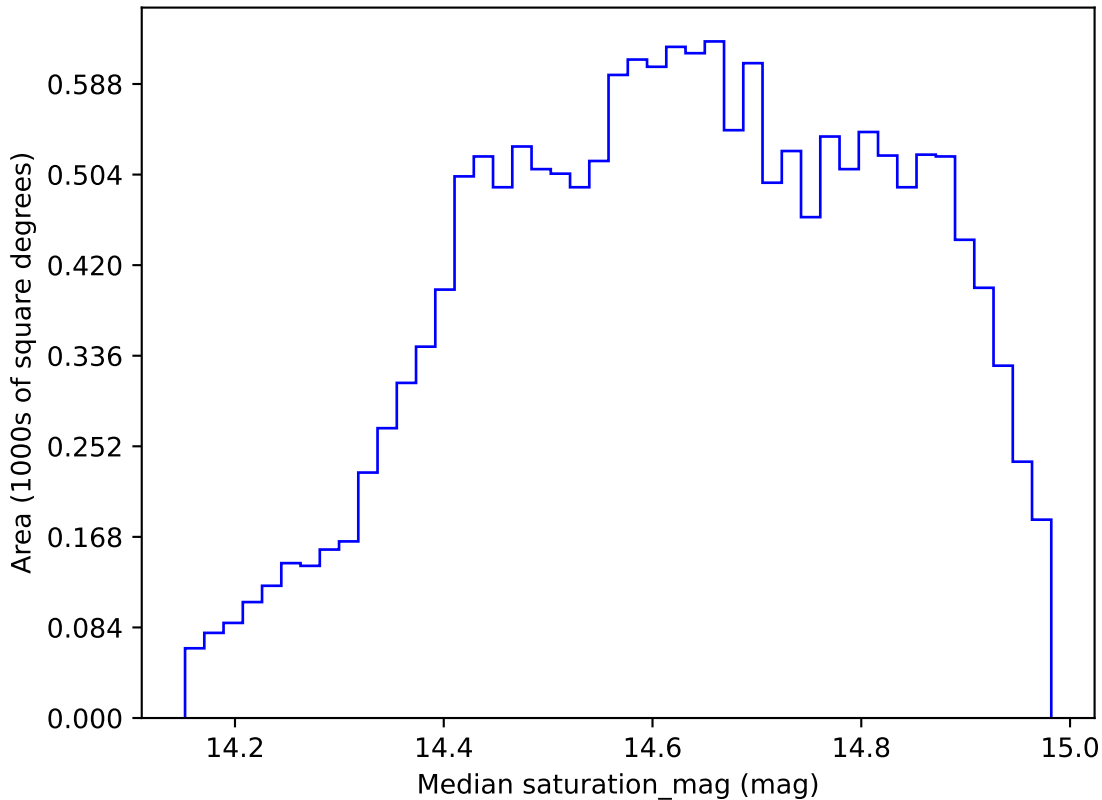
too_elab_r128_d3_gz_v3.4_10yrs WFD r band: Median saturation_mag
