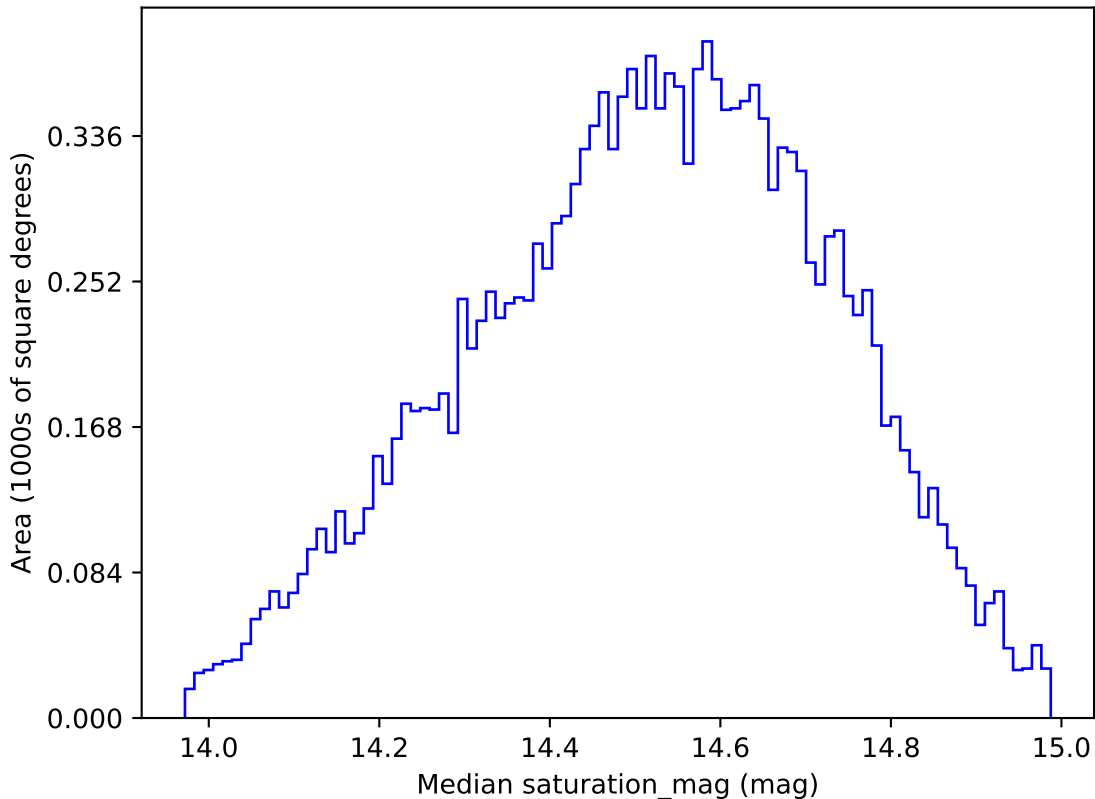
too_elab_r128_d3_gz_v3.4_10yrs WFD g band: Median saturation_mag
