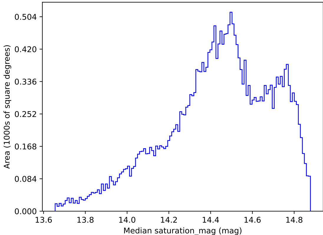
too_elab_r128_d3_gz_v3.4_10yrs All sky i band: Median saturation_mag
