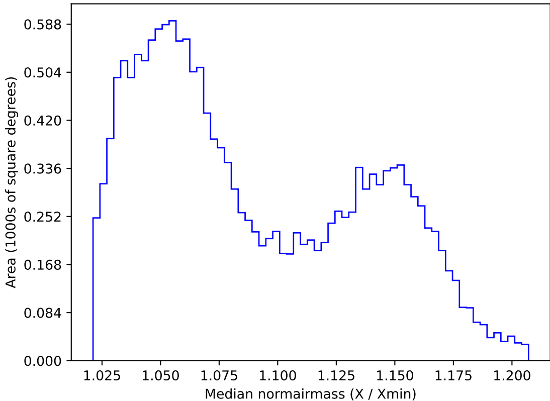
too_elab_r128_d3_gz_v3.4_10yrs WFD z band: Median normairmass
