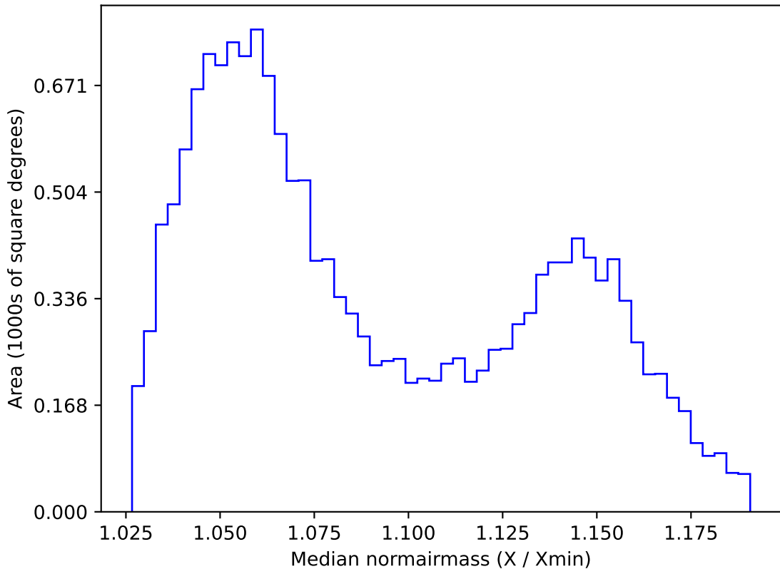
too_elab_r128_d3_gz_v3.4_10yrs WFD y band: Median normairmass
