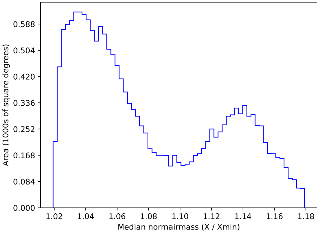
too_elab_r128_d3_gz_v3.4_10yrs WFD i band: Median normairmass
