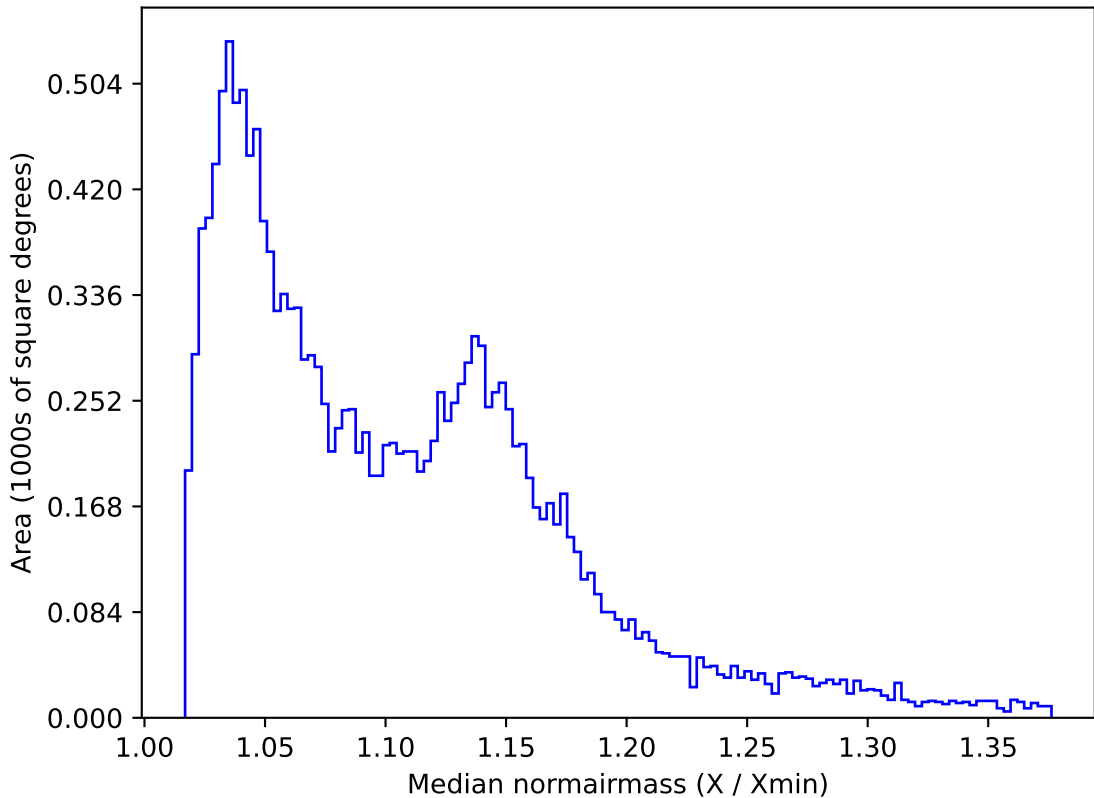
too_elab_r128_d3_gz_v3.4_10yrs WFD g band: Median normairmass
