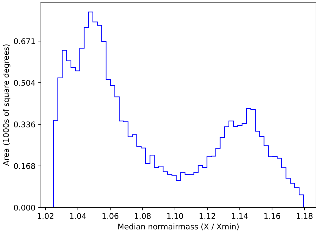
too_elab_r128_d3_gz_v3.4_10yrs WFD all bands: Median normairmass
