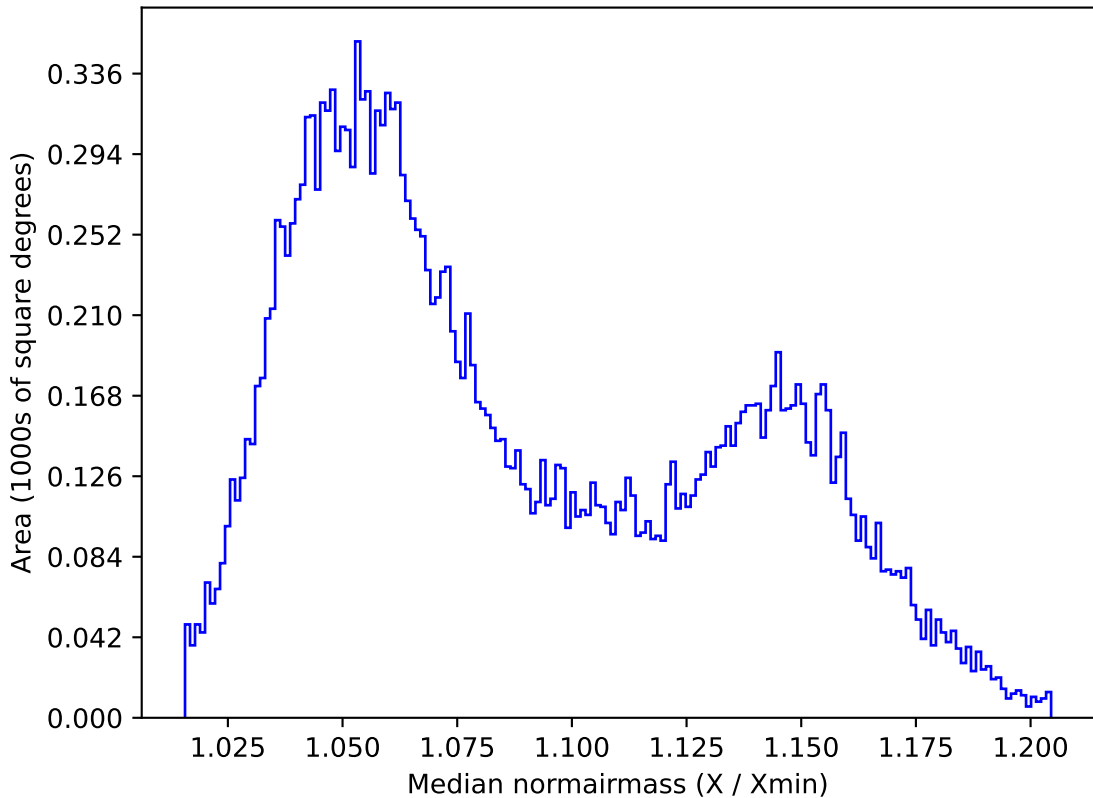
too_elab_r128_d3_gz_v3.4_10yrs All sky y band: Median normairmass
