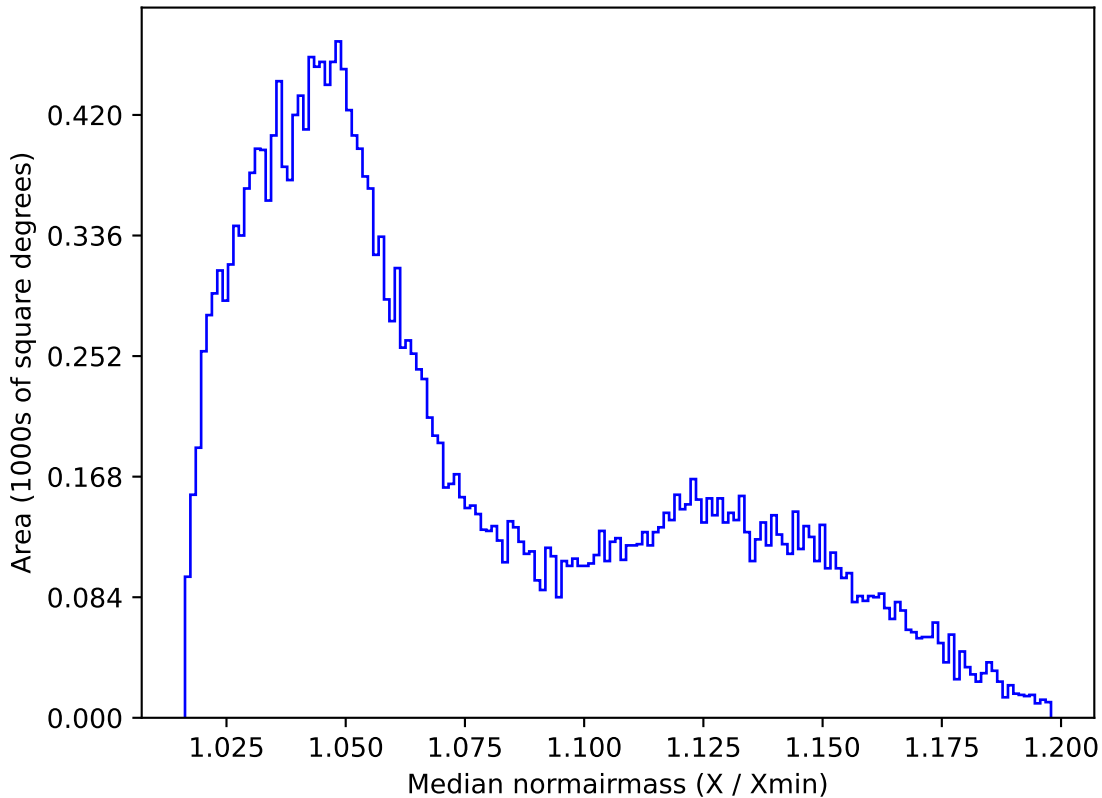
too_elab_r128_d3_gz_v3.4_10yrs All sky r band: Median normairmass
