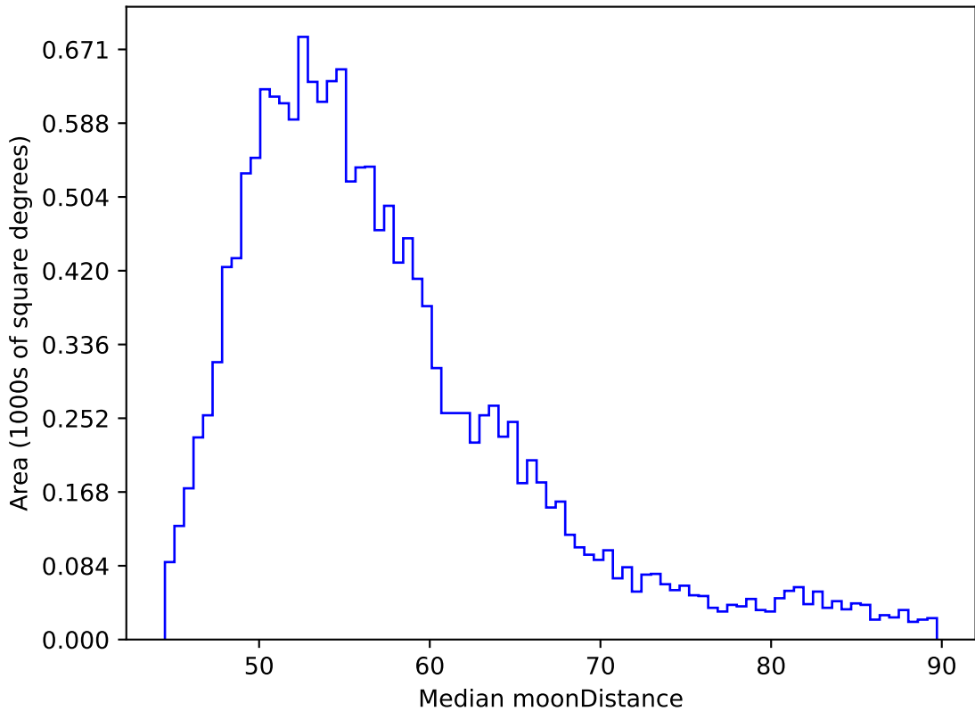
too_elab_r128_d3_gz_v3.4_10yrs WFD y band: Median moonDistance
