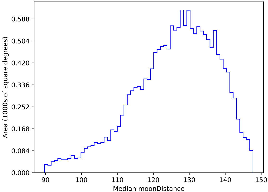
too_elab_r128_d3_gz_v3.4_10yrs WFD u band: Median moonDistance
