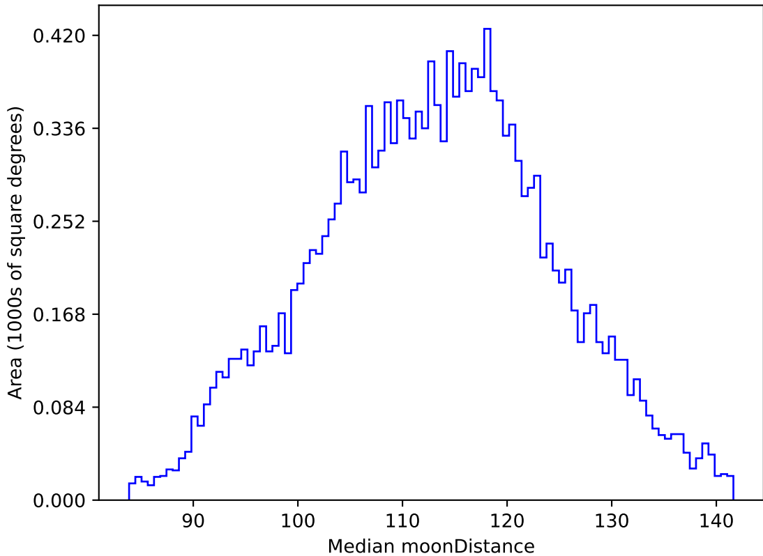
too_elab_r128_d3_gz_v3.4_10yrs WFD g band: Median moonDistance
