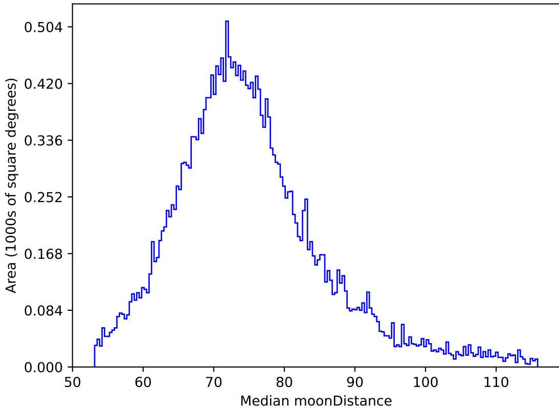
too_elab_r128_d3_gz_v3.4_10yrs All sky z band: Median moonDistance
