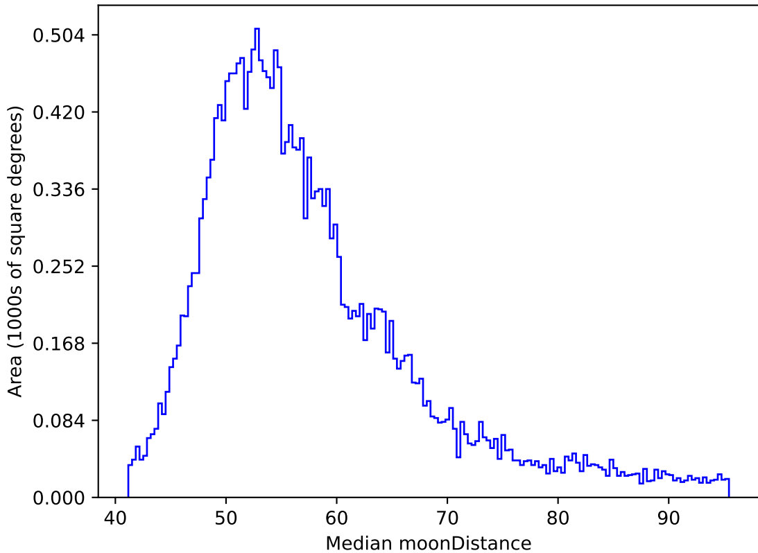
too_elab_r128_d3_gz_v3.4_10yrs All sky y band: Median moonDistance
