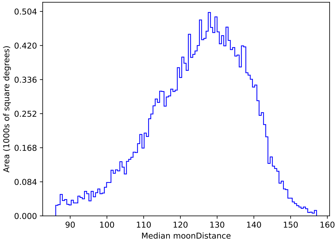
too_elab_r128_d3_gz_v3.4_10yrs All sky u band: Median moonDistance
