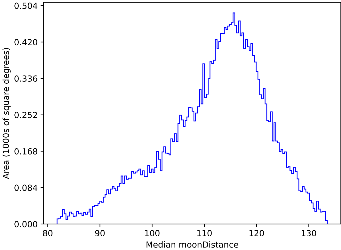
too_elab_r128_d3_gz_v3.4_10yrs All sky r band: Median moonDistance
