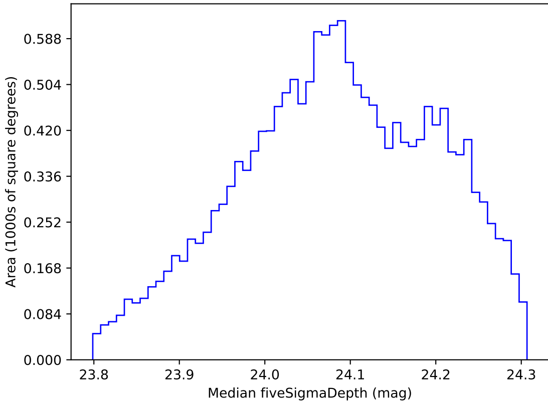
too_elab_r128_d3_gz_v3.4_10yrs WFD r band: Median fiveSigmaDepth
