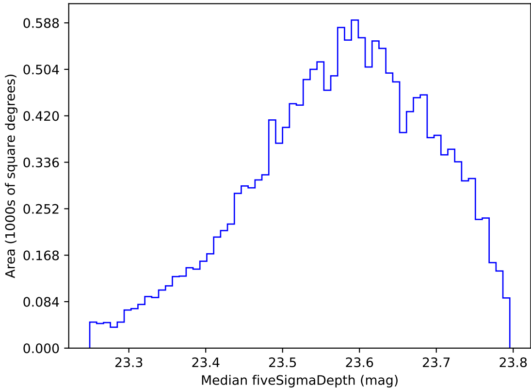
too_elab_r128_d3_gz_v3.4_10yrs WFD i band: Median fiveSigmaDepth
